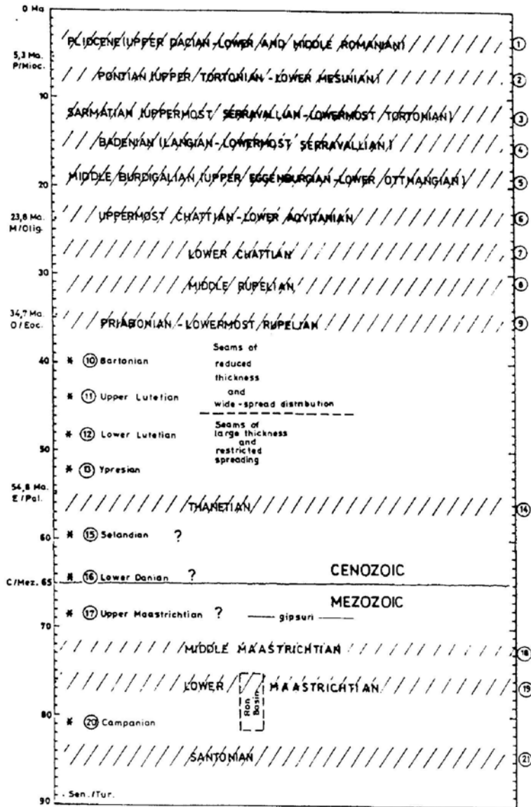
Fig. 1 The coal-generating phases of Santonian-Pliocene in Parathetys
